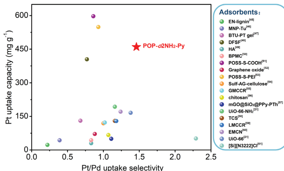
Figure 2. Comparison of platinum equilibrium uptake capacity as a function of Pt/Pd uptake selectivity of POP-oNH 2 -Py with that of other benchmark sorbent systems (refer to detailed information of samples in Table S1, Supporting Information).
