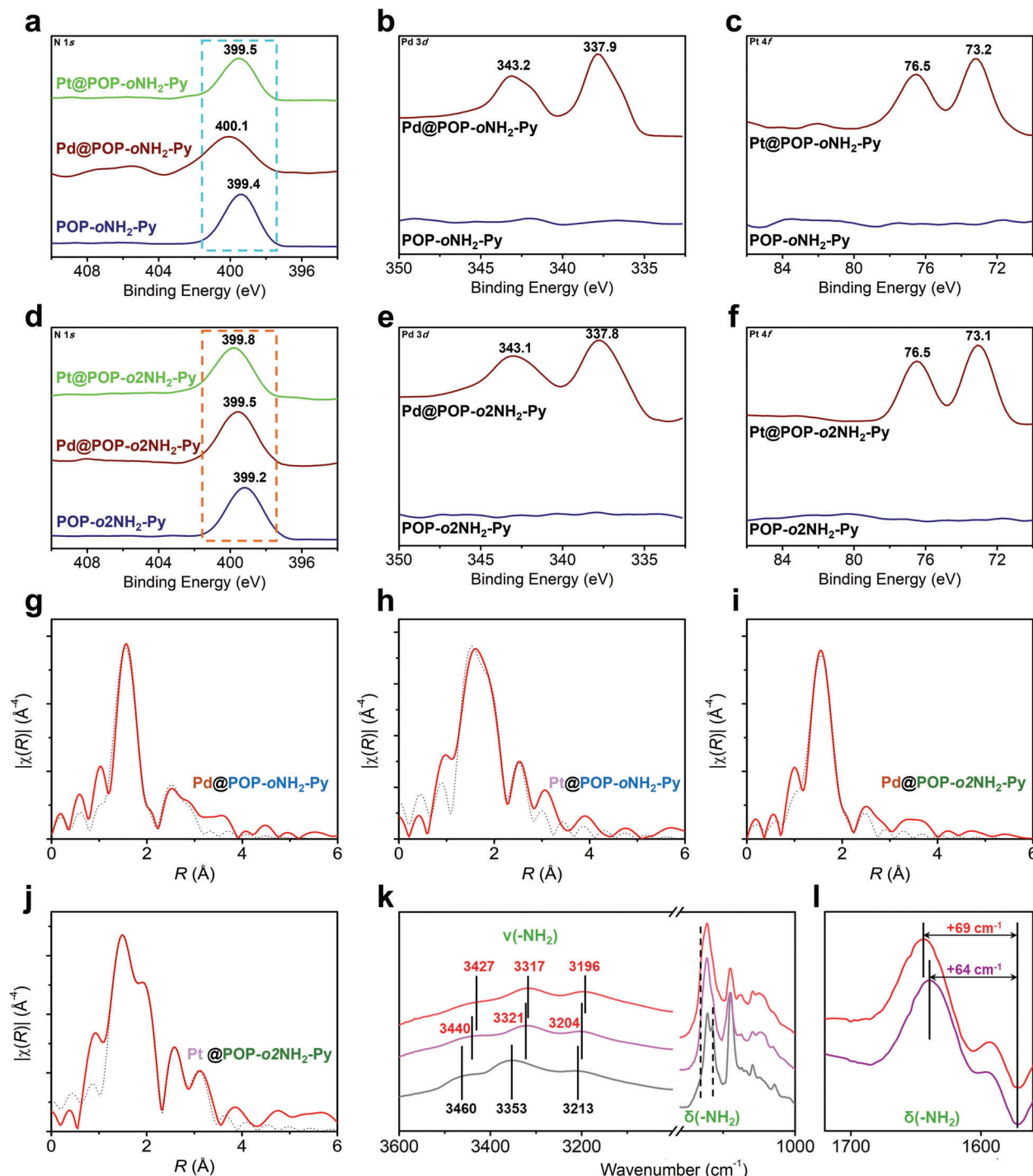
Figure 3. Binding mechanism investigation. a–c) XPS spectra of POP-oNH 2 -Py treated by palladium or platinum. d–f) XPS spectra of POP-o2NH 2 -Py treated by palladium or platinum. g, h) EXAFS spectra of palladium and platinum loaded POP-oNH 2 -Py. i, j) EXAFS spectra of palladium and platinum loaded POP-o2NH 2 -Py. k) IR spectra of pristine (gray), Pd- (purple) and Pt- (red) loaded POP-o2NH 2 -Py, and l) shows the difference spectra in the region 1720–1560 cm -1 obtained by subtracting the spectrum of pristine POP-o2NH 2 -Py from Pd- (purple) and Pt- (red) loaded one.
